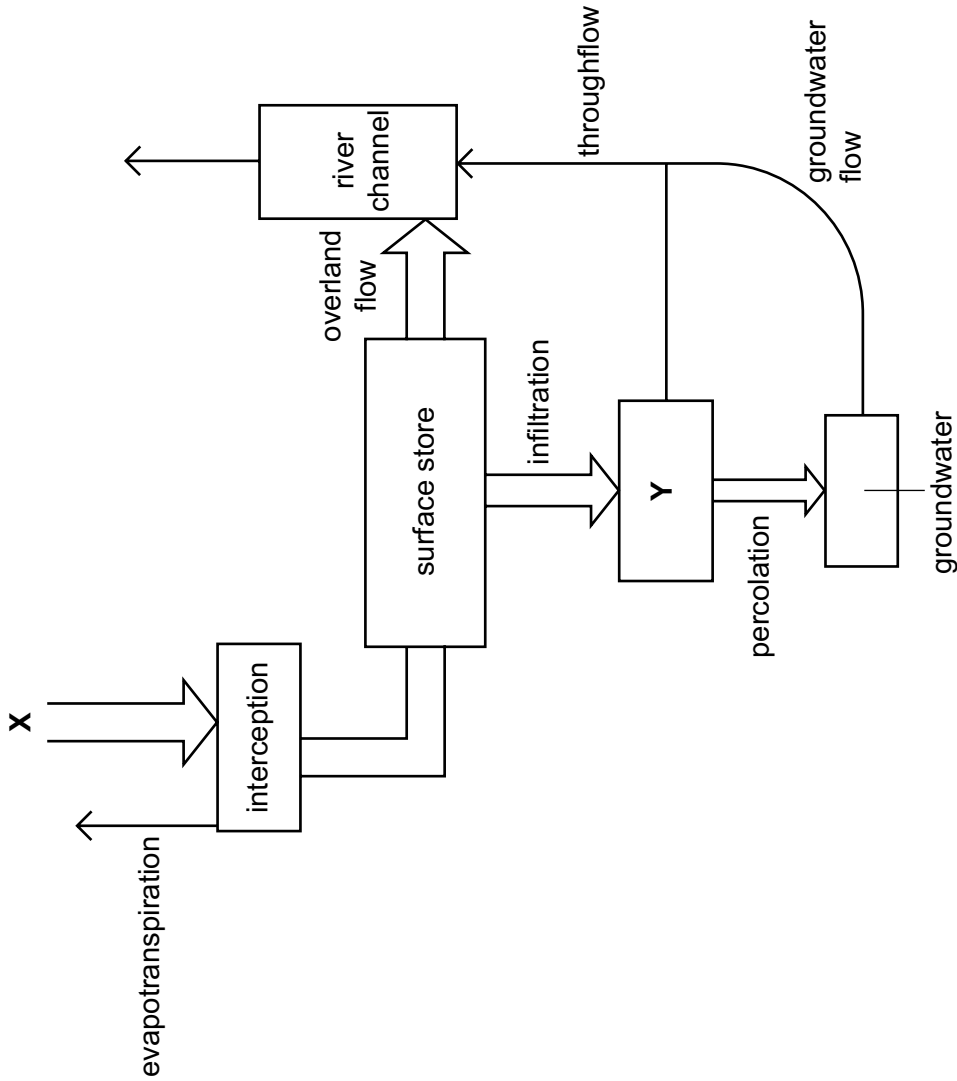
Schematic diagram of drainage basin systems in Tropical Savannah climate zone during the wet season
